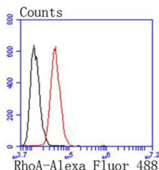
Fig. 3. Flow cytometric analysis of HeLa cells with RhoA antibody at 1/50 dilution (red) compared with an unlabelled control (cells without incubation with primary antibody; black). Alexa Fluor 488-conjugated goat anti rabbit IgG was used as the secondary antibody.
